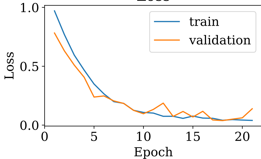
Loss
