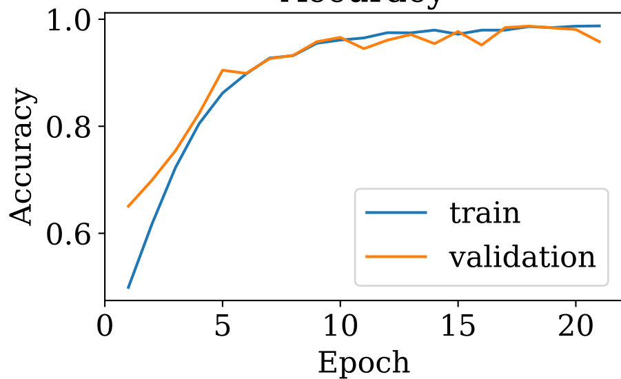
Accuracy
