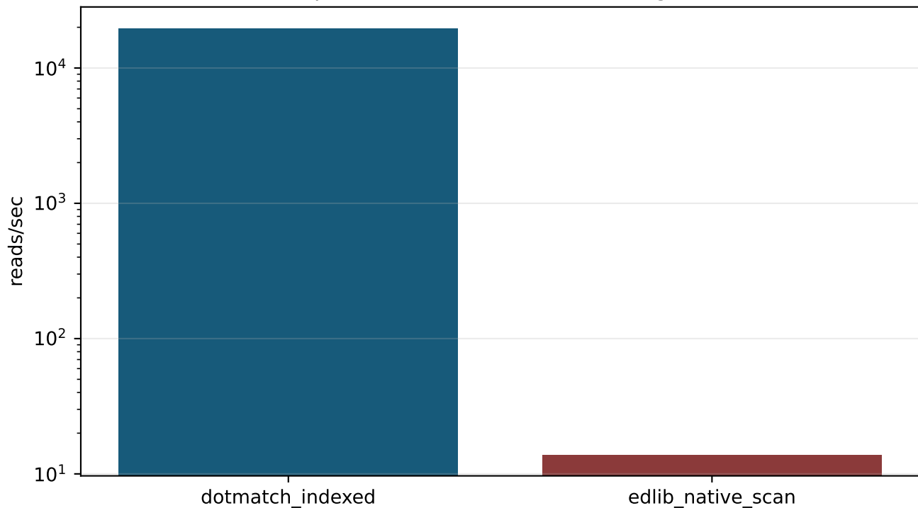
Real public CRISPR reads: k=1 assignment
