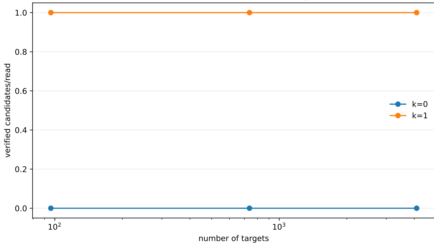
DotMatch indexed candidates verified per read
