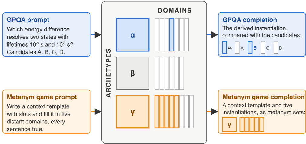
Figure 3: A hypothesis for the 0.98: the metonymy game reproduces the way the model organises its knowledge, and GPQA runs on that organisation. An archetype ( \alpha , \beta , \gamma ) is held once, about eight times the size of a domain’s instantiation (the slices); each domain adds only its metonym set. GPQA: archetype and domain are given; the model derives the instantiation and selects the matching candidate. The game: nothing is given; the model selects the archetype and domains that best satisfy the criteria and writes them out.
