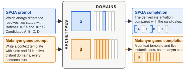
Figure 7: A hypothesis for the 0.98: the metonym game reproduces the way the model organises its knowledge, and GPQA runs on that organisation. An archetype ( \alpha , \beta ) is held once; each domain adds only its metonym set (the slices), about a fifth of the instantiation it yields. GPQA: archetype and domain are given; the model derives the instantiation and selects the matching candidate. The game: nothing is given; the model selects the archetype and domains that best satisfy the criteria and writes them out.
