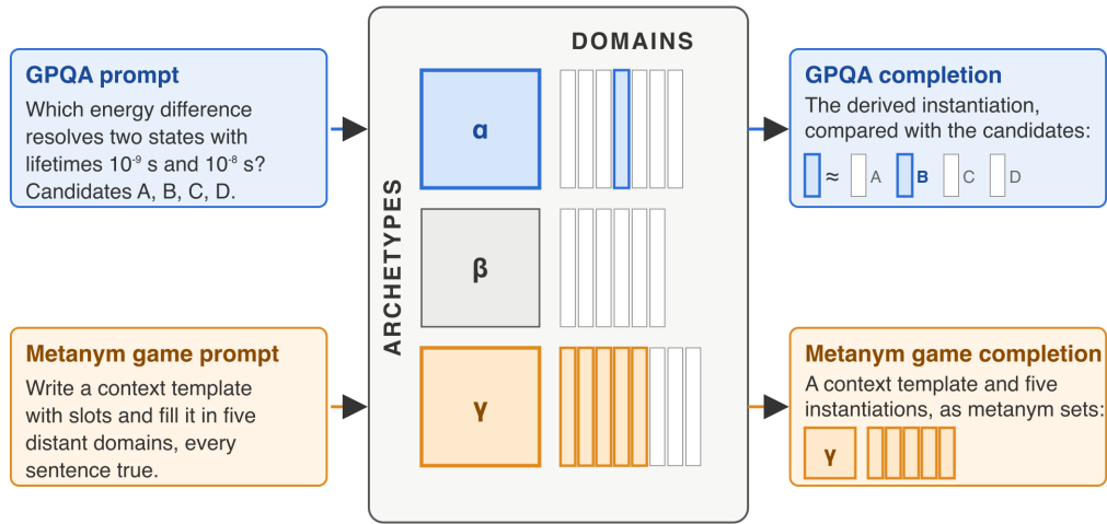
Figure 7: A hypothesis for the 0.98: the metonym game reproduces the way the model organises its knowledge, and GPQA runs on that organisation. An archetype ( \alpha , \beta , \gamma ) is held once; each domain adds only its metonym set (the slices), about a fifth of the instantiation it yields. GPQA: archetype and domain are given; the model derives the instantiation and selects the matching candidate. The game: nothing is given; the model selects the archetype and domains that best satisfy the criteria and writes them out.
