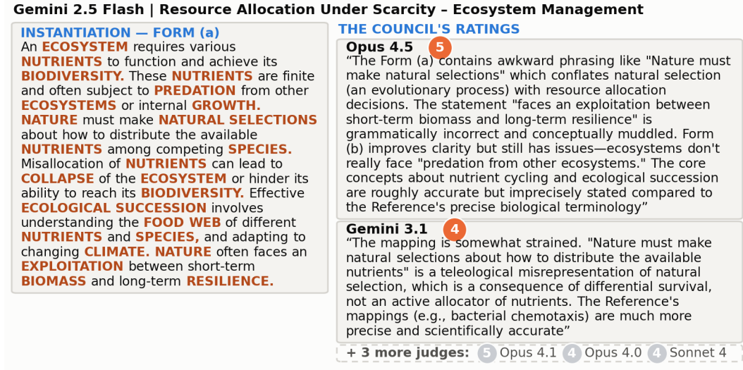
Figure 1: One parallel context under evaluation: the instantiation with its metonyms marked, and the five judges' ratings with the clause each one singles out. All five isolate the same clause; the disagreement that remains, 4 versus 5, is about severity. The whole evaluation, with the rewrite, the administrator's synthesis and every justification, is Figure 4 in Appendix C.
