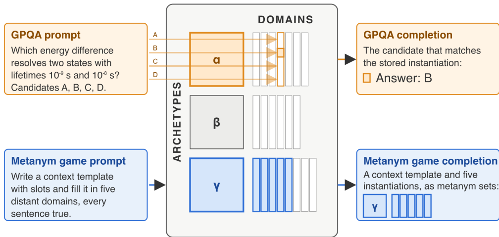
Figure 3: A hypothesis for the 0.98 correlation between the GPQA and Metanym Game benchmarks: the metanym game reproduces the way the model organises its knowledge, and GPQA runs on that organisation. An archetype ( \alpha , \beta , \gamma ) is held once, about eight times the size of a domain’s instantiation (the slices); each domain adds only its metanym set. GPQA offers four candidate instantiations, and the completion is the one that matches what is stored: the mechanism in use. The game offers nothing, and the completion is an archetype with five instantiations: the mechanism itself.
