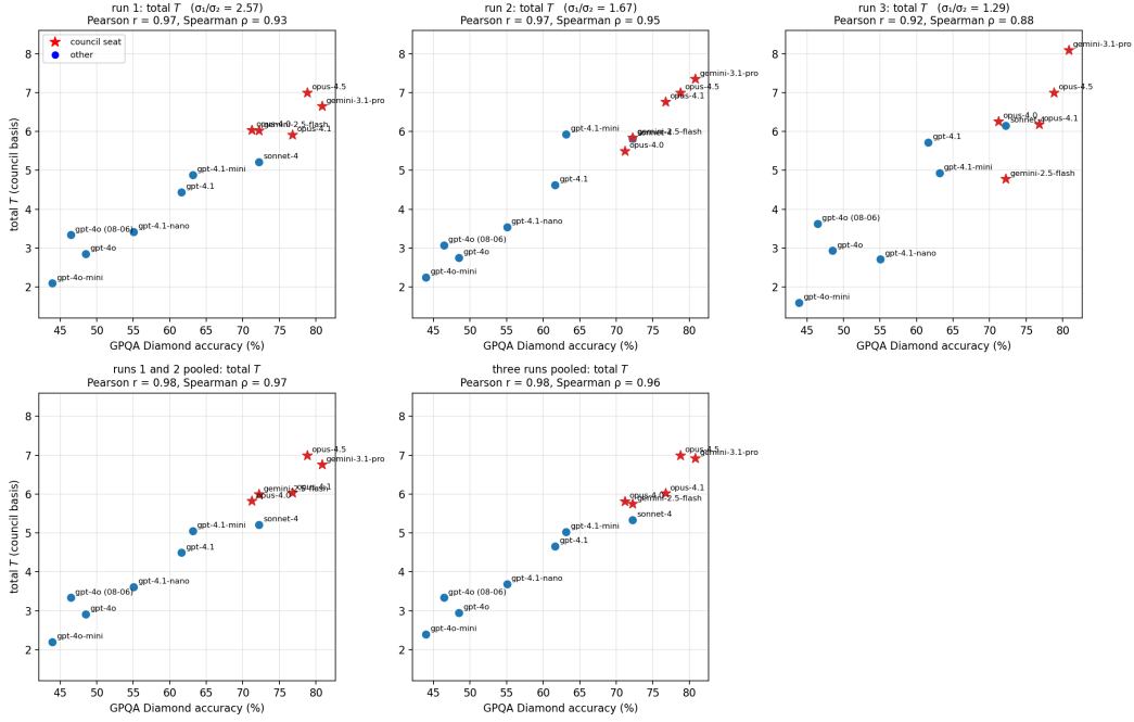
Figure 3: The three runs apart and pooled, against GPQA Diamond. Top row: council-basis T per run, with each run’s twelve-evaluator spectral gap. Bottom row: runs 1 and 2 pooled (left), all three pooled (right). Run 3, with the smallest gap, is the odd one out; pooling restores an identified factual axis and the agreement rises.
