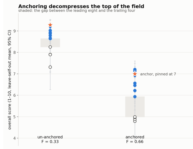
Figure 7: Each model’s leave-self-out overall mean with its 95% bootstrap CI, un-anchored (left) and anchored (right); models are unlabelled deliberately — the message is structural, not a ranking. Filled markers are the leading eight, open the trailing four, the shaded band the gap between them; the star is the anchor — a scored target on the left, the pinned reference (7) on the right. Anchored scores spread around the yardstick instead of piling against the ceiling: the gap more than doubles relative to the spread of the means (every scored cross-band pair holds at bootstrap probability 1.00), the variance ratio — between-target over within-target variance, Fisher’s F — doubles from 0.33 to 0.66, and the intervals still overlap within each band.
