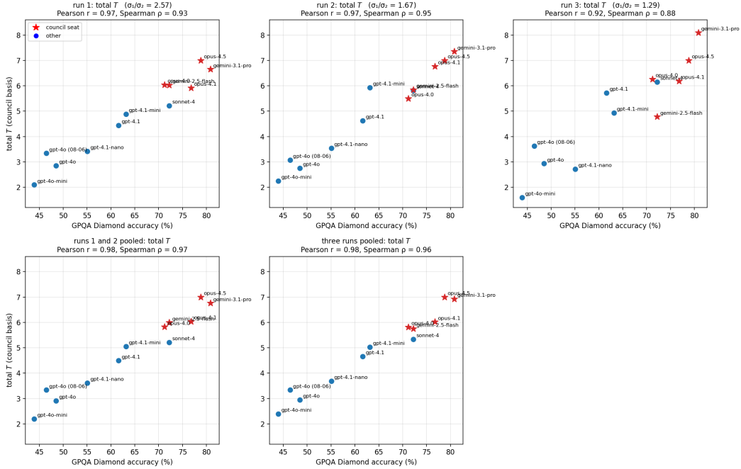
Figure 6: The three runs apart and pooled, against GPQA Diamond. Top row: council-basis T per run, with each run’s twelve-evaluator spectral gap. Bottom row: runs 1 and 2 pooled (left), all three pooled (right). Run 3, with the smallest gap, is the odd one out; pooling restores an identified factual axis and the agreement rises.
