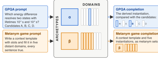
Figure 7: A hypothesis for the 0.98: the metanym game reproduces the way the model organises its knowledge, and GPQA runs on that organisation. An archetype ( \alpha , \beta ) is held once; each domain adds only its metanym set (the slices), about a fifth of the instantiation it yields. GPQA: archetype and domain are given; the model derives the instantiation and selects the matching candidate. The game: nothing is given; the model selects the archetype and domains that best satisfy the criteria and writes them out.
