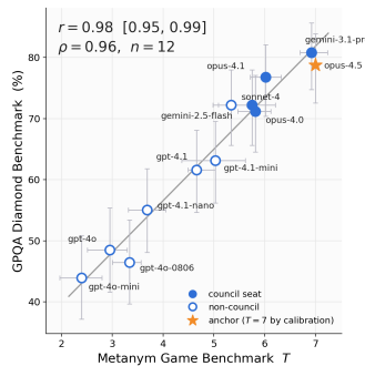
Figure 7: The agreement the hypothesis is offered for, reproduced from Figure 2: the official total T (council basis, three runs pooled) against self-administered GPQA Diamond accuracy, twelve models; Pearson r = 0.98 (95% BCa CI [0.95, 0.99]), Spearman \rho = 0.96 . Filled markers are council seats, open markers non-council, the star the anchor at T = 7 by calibration.
