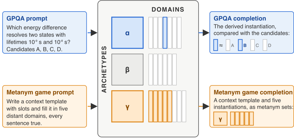
Figure 3: A hypothesis for the 0.98: the metanym game reproduces the way the model organises its knowledge, and GPQA runs on that organisation. An archetype ( \alpha , \beta , \gamma ) is held once, about eight times the size of a domain’s instantiation (the slices); each domain adds only its metanym set. GPQA: archetype and domain are given; the model derives the instantiation and selects the matching candidate. The game: nothing is given; the model selects the archetype and domains that best satisfy the criteria and writes them out.
