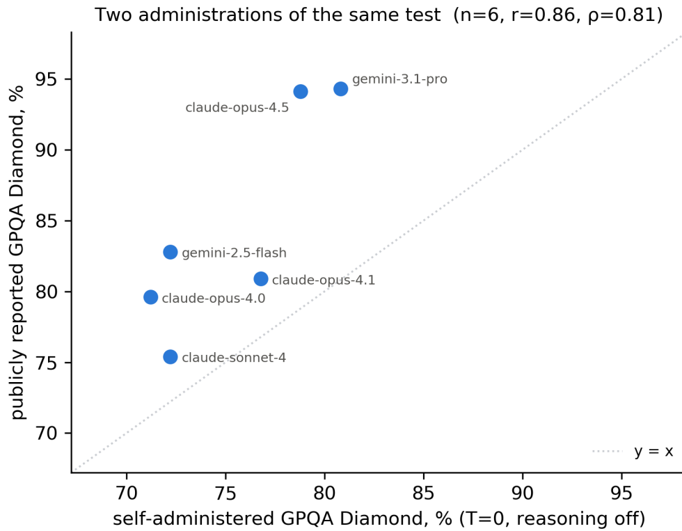
Figure 4. Two administrations of the same test: publicly reported GPQA Diamond (typically reasoning-on) against this protocol's self-administered accuracy (T=0, reasoning off), for the six models with a citable public value. Pearson r = 0.86 , Spearman \rho = 0.81 . The offset above the diagonal is the reasoning budget. Produced by scripts/plot_gpqa_public_vs_measured.py .
