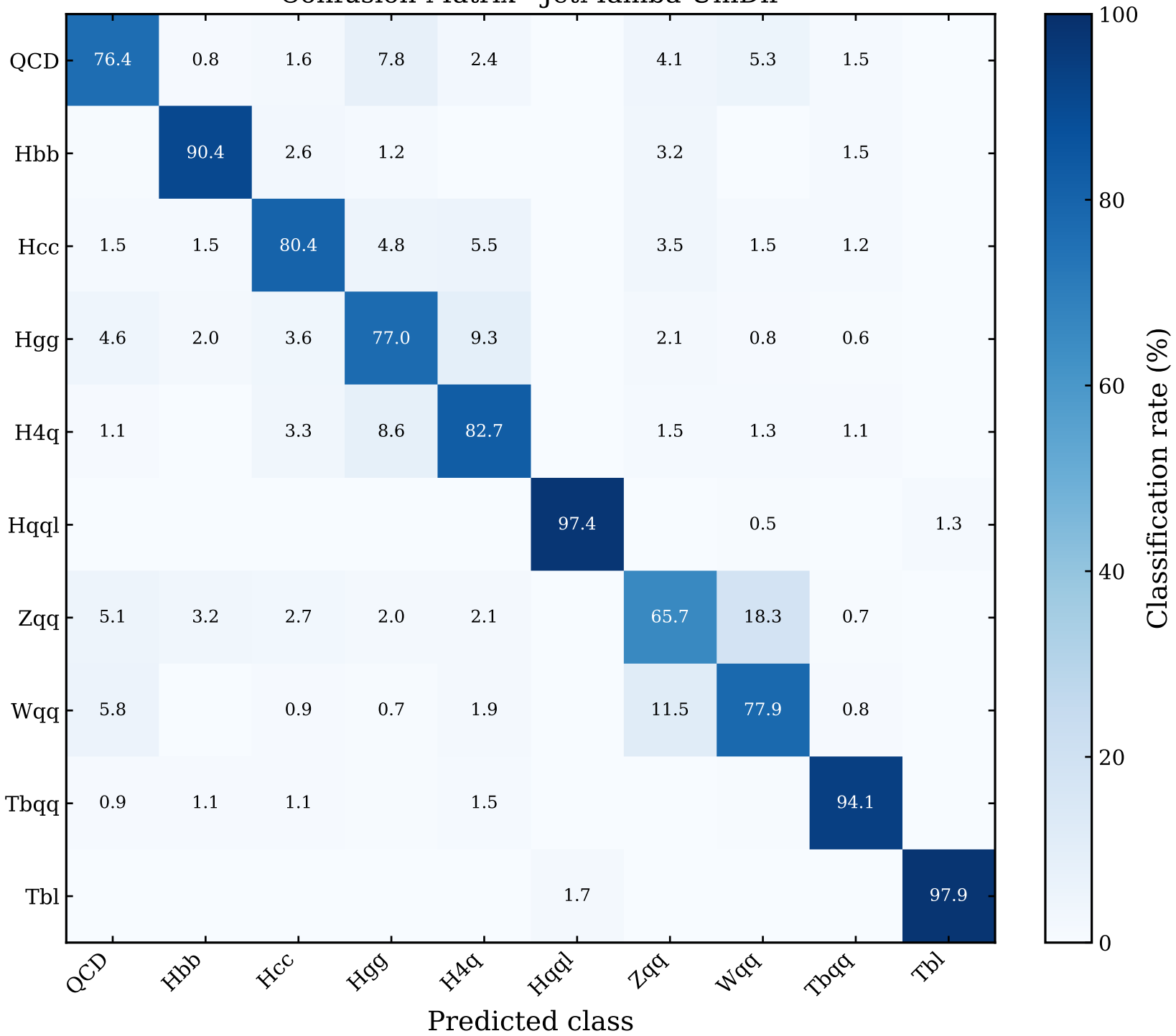
Confusion Matrix - JetMamba-UniDir
