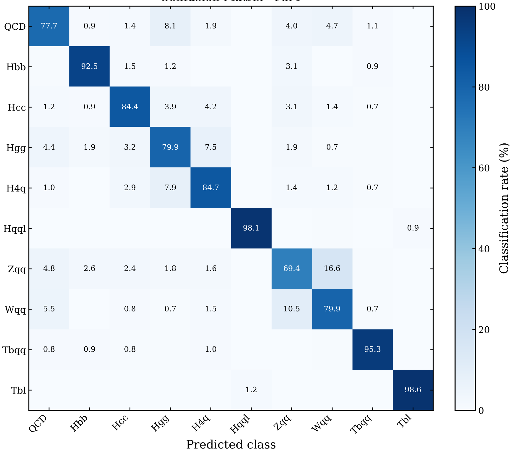
Confusion Matrix - ParT
