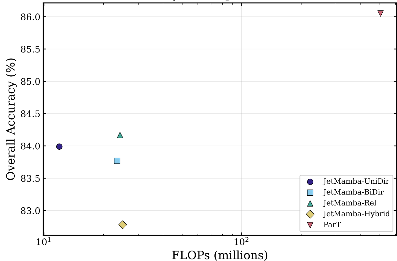
Accuracy vs Computational Cost
