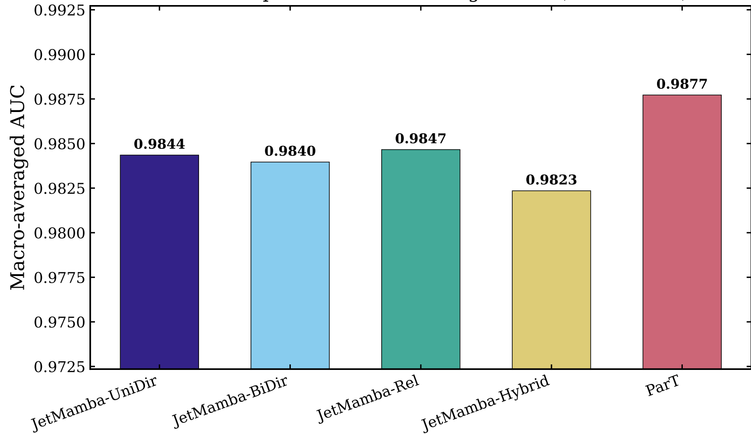
Model Comparison: Macro-averaged AUC (One-vs-Rest)
