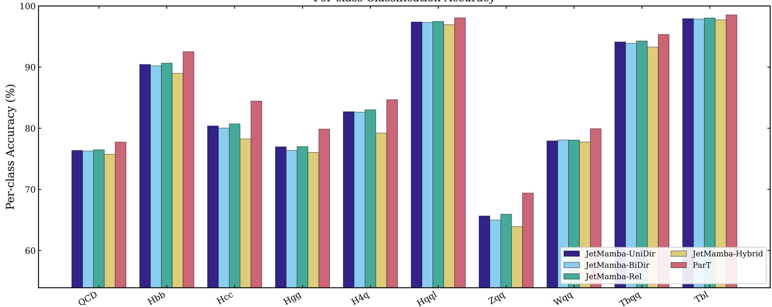
Per-class Classification Accuracy
