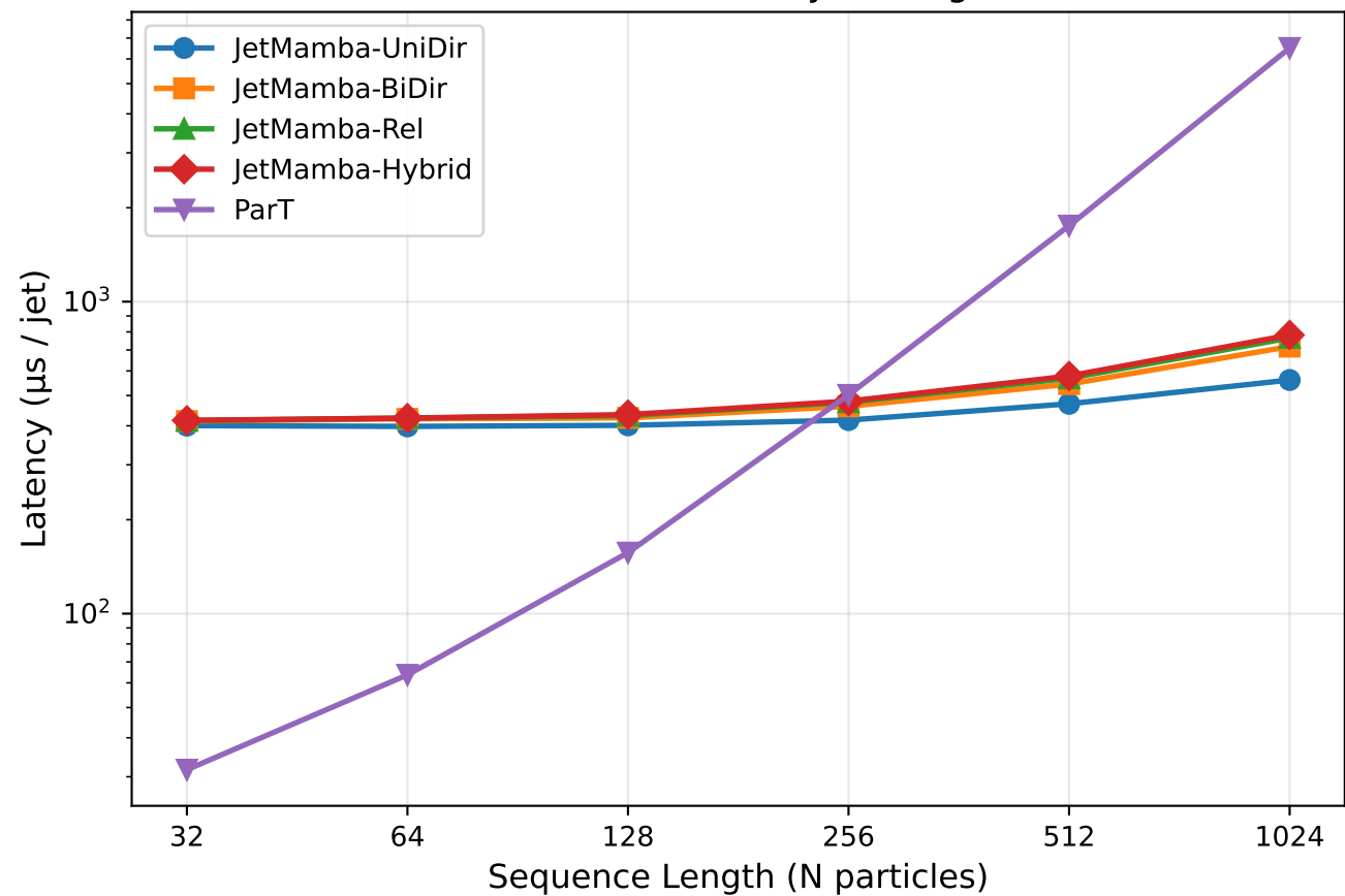
Inference Latency Scaling
