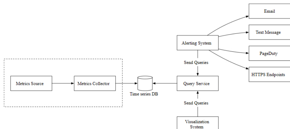
Figure 7 Metrics collection flow
