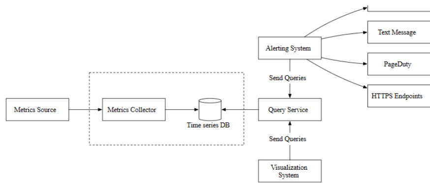
Figure 14 Metrics transmission pipeline
