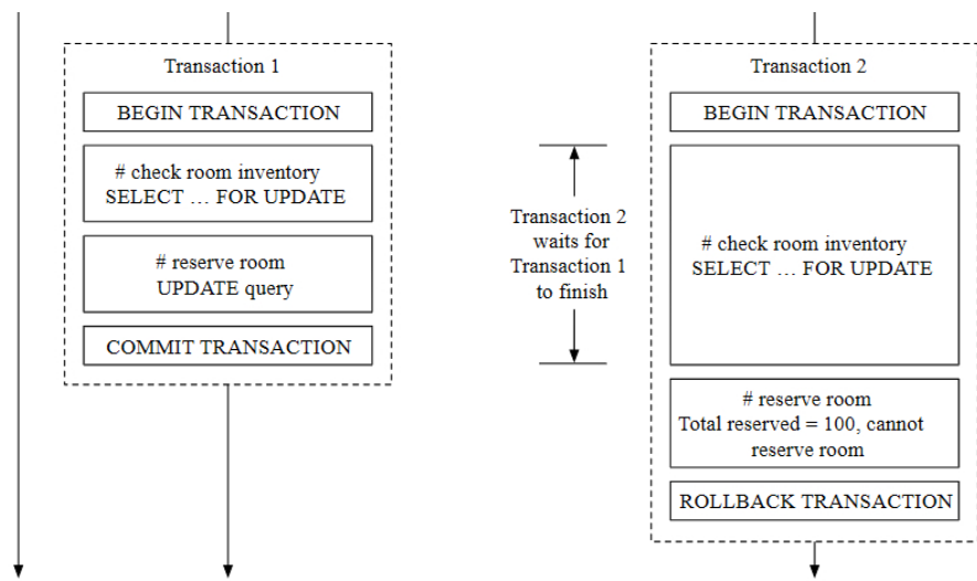
Figure 12 Pessimistic locking
