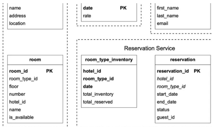
Figure 6 Updated schema
