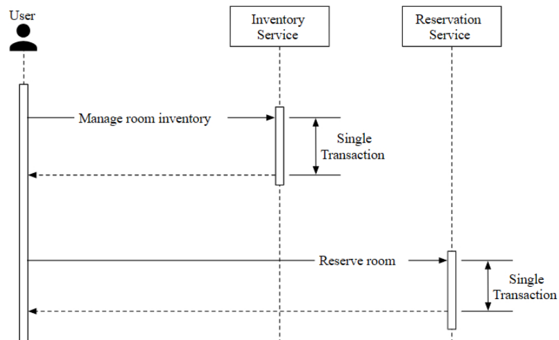
Figure 19 Microservice architecture
