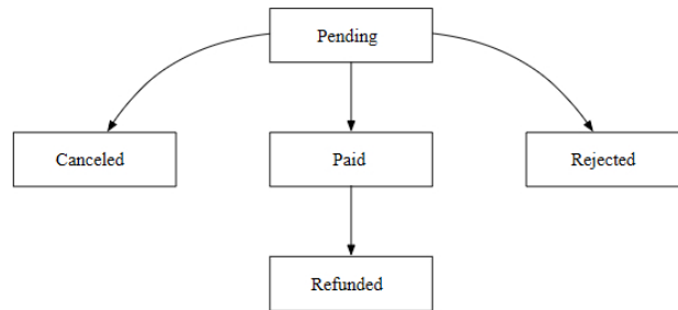
Figure 3 Reservation status
