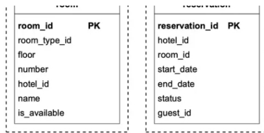
Figure 2 Database schema
