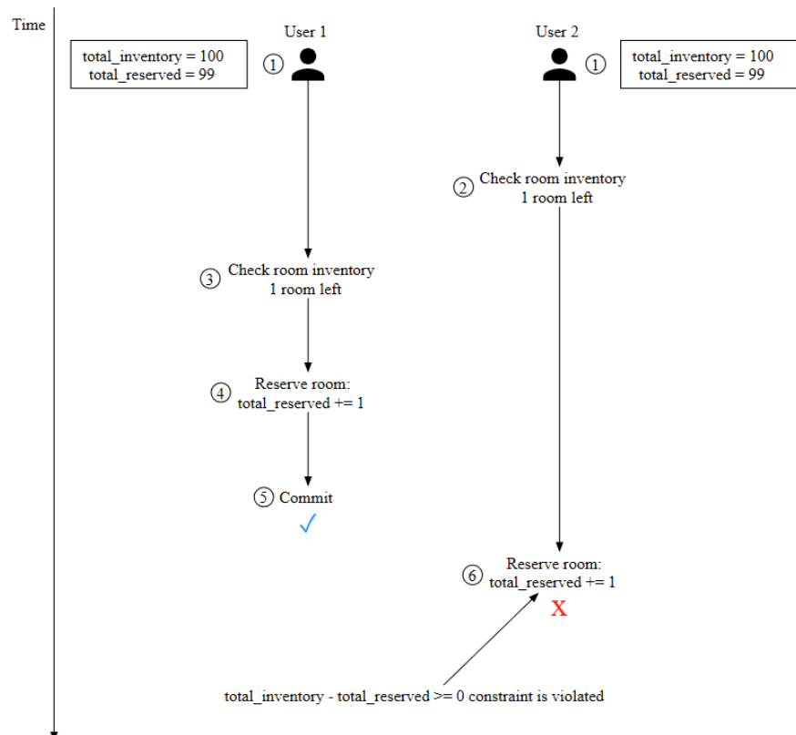
Figure 14 Database constraint
