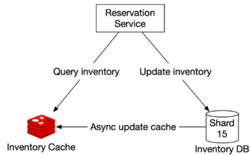
Figure 16 Caching
