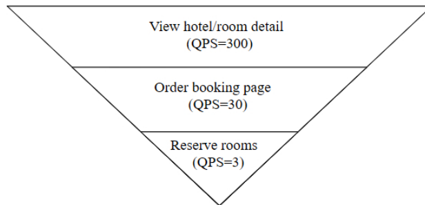
Figure 1 QPS distribution
