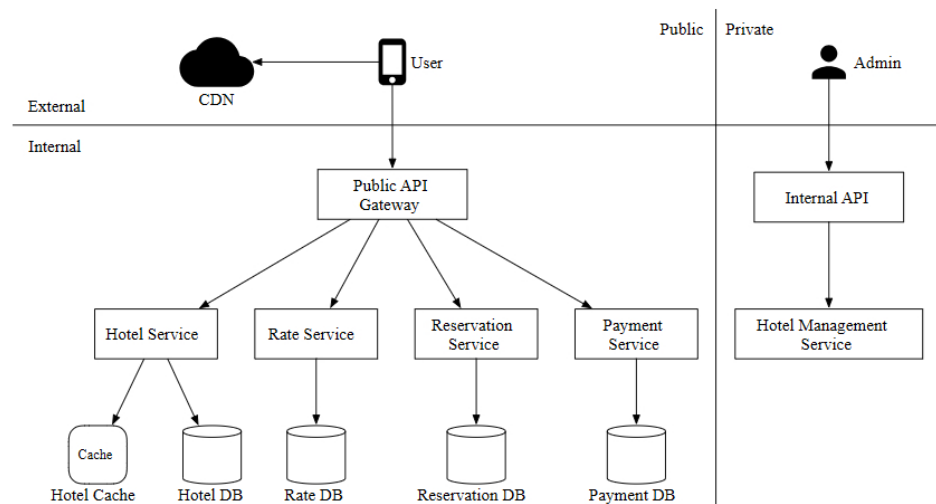
Figure 4 High-level design
