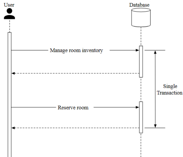
Figure 18 Monolithic architecture
