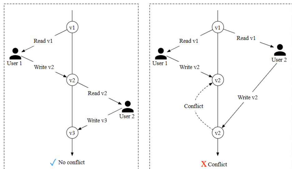
Figure 13 Optimistic locking
