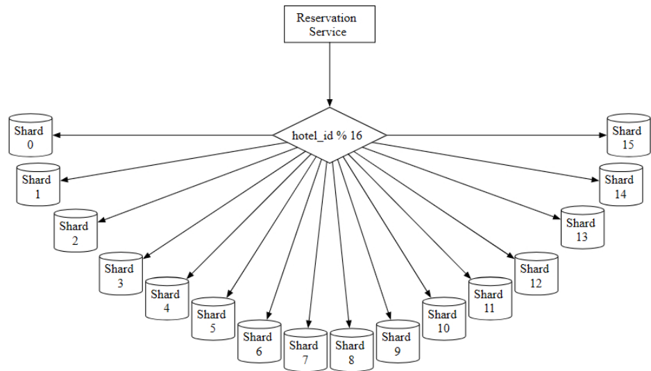
Figure 15 Database sharding
