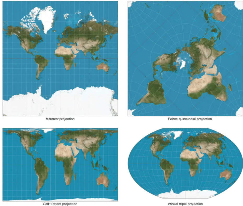
Figure 2 Map projections (source: Wikipedia [6] [7] [8] [9])
