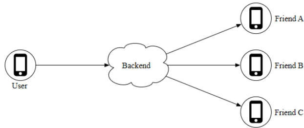
Figure 3 Shared backend
