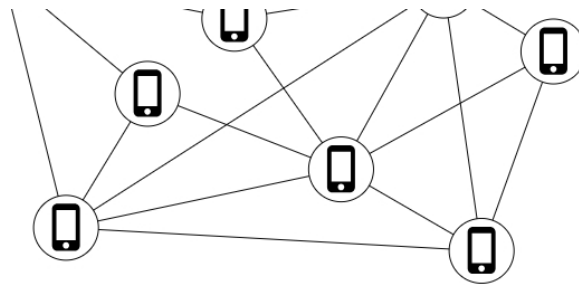
Figure 2 Peer-to-peer
