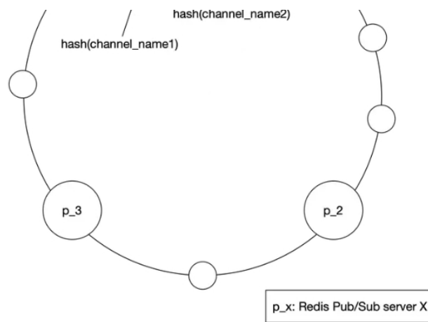
Figure 9 Consistent hashing
