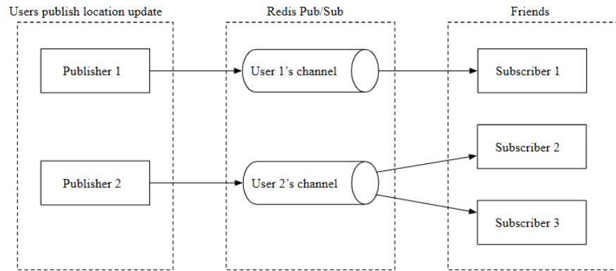
Figure 6 Redis Pub/Sub
