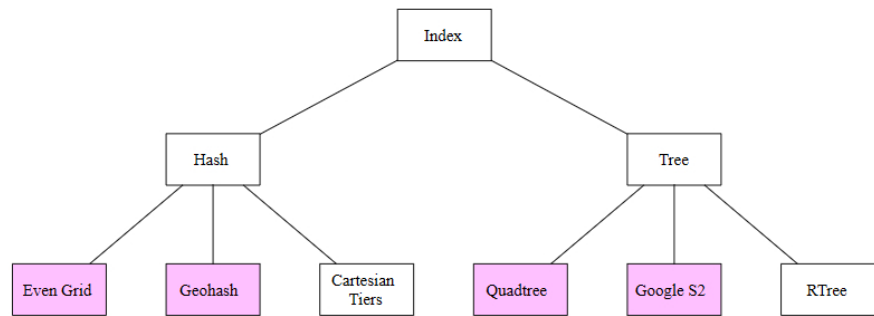
Figure 5 Different types of geospatial indexes
