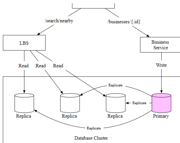
Figure 2 High-level design
