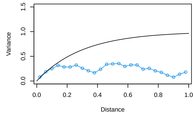
Empirical Variogram
