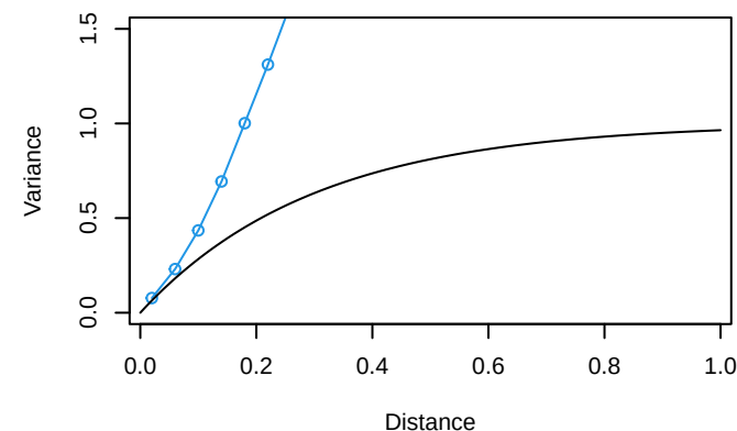
Empirical Variogram
