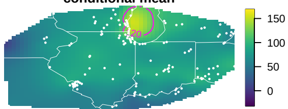
conditional mean
