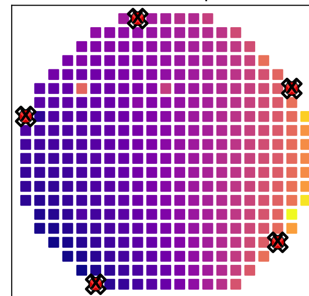
Max Comp
