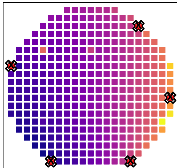
Min Comp
