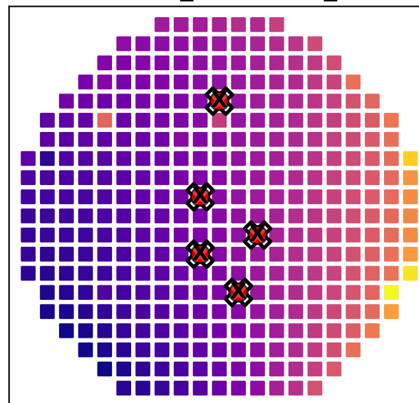
Centroids_saturation_low
