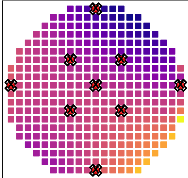
Four-point probe measurement
