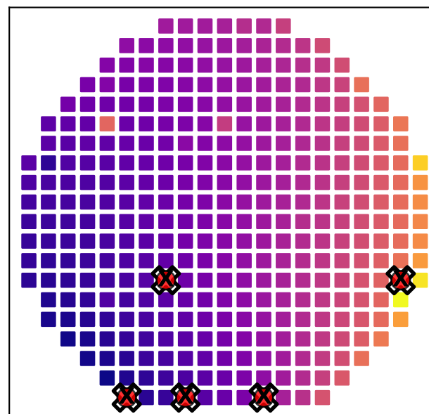
K-Means
