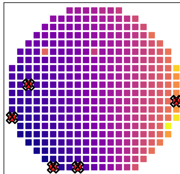
K-Center
