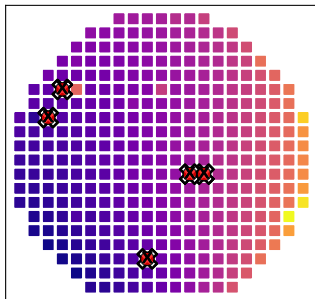
Random
