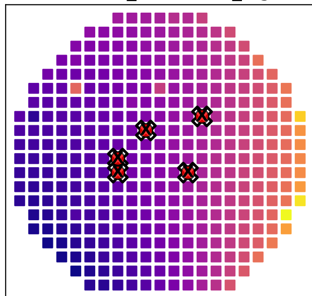
Centroids_saturation_high
