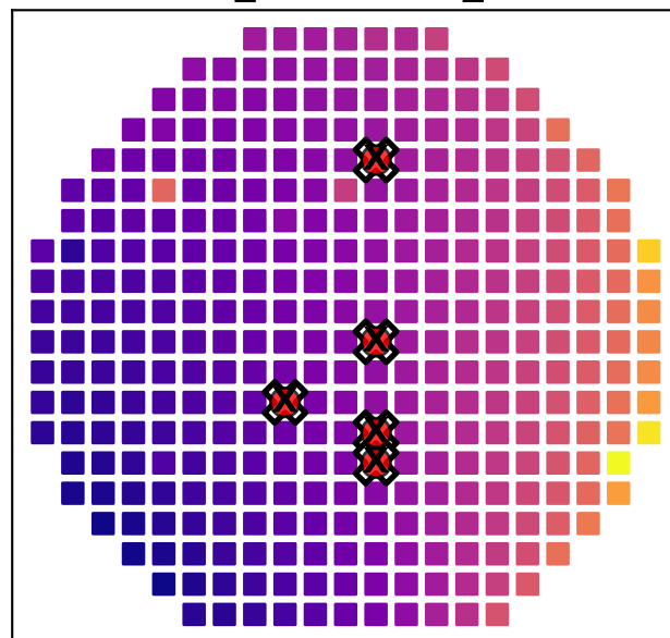
Centroids_saturation_medium
