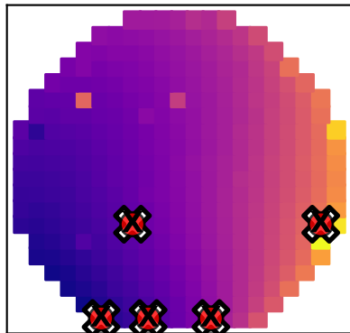
K-Means
