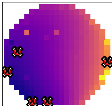
K-Center
