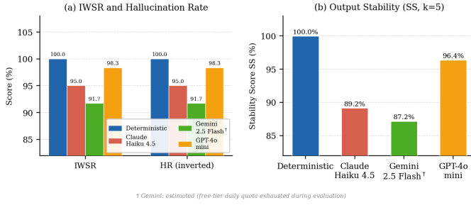
Fig. 5. Multi-LLM reliability comparison across four configurations. Panel (a) shows IWSR and hallucination rate (HR, inverted: 100 % – HR). Panel (b) shows output stability (SS, k = 5 repeated runs). SCR and SVR reach 100 % in all LLM-assisted configurations due to schema-grounded Phase 2 prompting. Gemini 2.5 Flash and GPT-4o-mini results represent preliminary single-run measurements.
