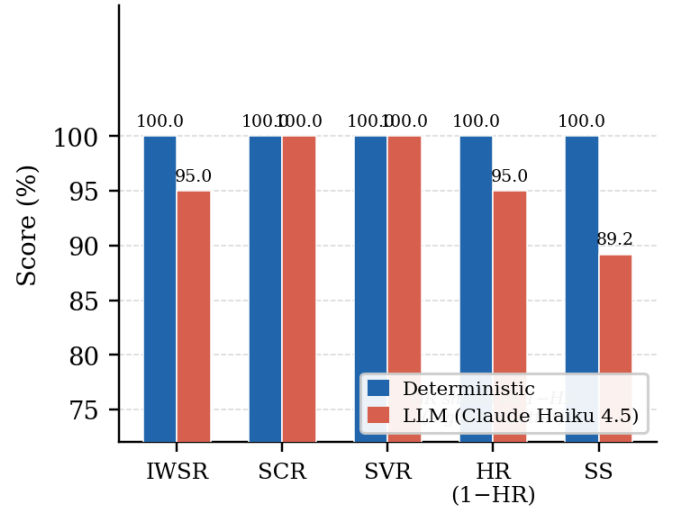
Fig. 2. Reliability metric comparison between deterministic and LLM-assisted modes across 60 evaluation entries. HR is displayed as 100 %–HR (inverted; higher is better). SCR and SVR are identical in both modes; the 5-point IWSR gap is entirely attributable to Phase 1 service-routing errors.
