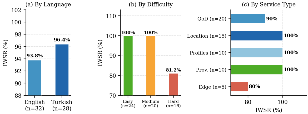
Fig. 3. IWSR breakdown by (a) language, (b) difficulty level, and (c) service type in LLM-assisted mode ( n = 60 ). Turkish entries marginally outperform English (96.4 % vs. 93.8 %), demonstrating cross-lingual generalisation without additional prompt engineering. Easy and medium entries achieve perfect IWSR; hard entries and edge cases expose Phase 1 routing ambiguity.
