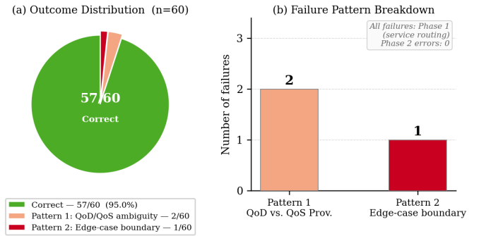
Fig. 4. LLM error analysis: (a) outcome distribution across 60 entries; (b) failure pattern breakdown. All 3 failures are Phase 1 service-routing errors; zero Phase 2 payload errors occur in any mode.
