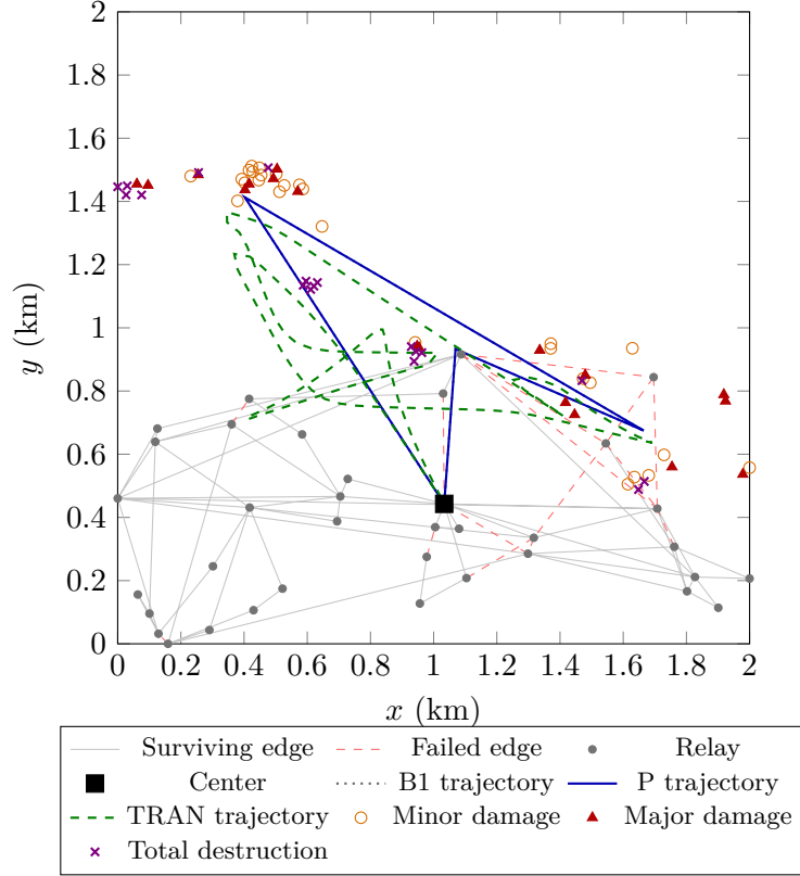
Figure 9. Targets, relay network, and UAV trajectories in the representative case-study scenario.
