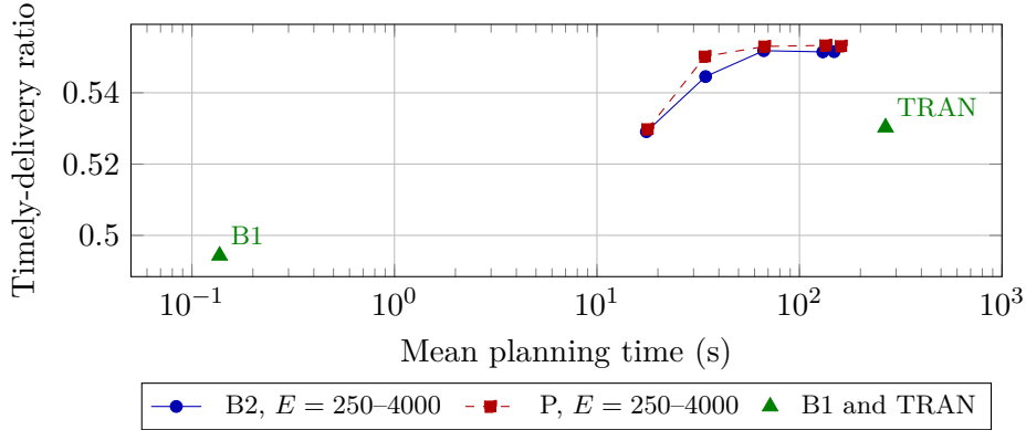
Figure 6. Timely-delivery ratio versus planning time on v0.
