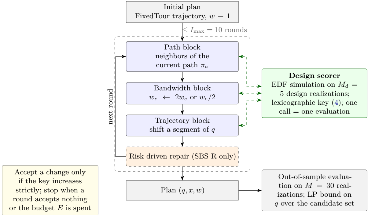
Figure 2. Pipeline of the proposed block search.
