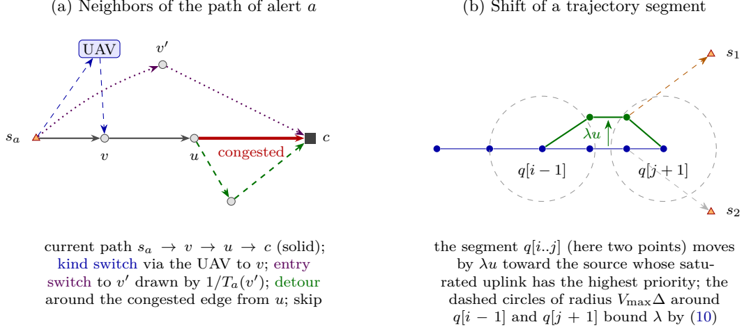
Figure 4. Neighborhoods of the path block and the trajectory block.
