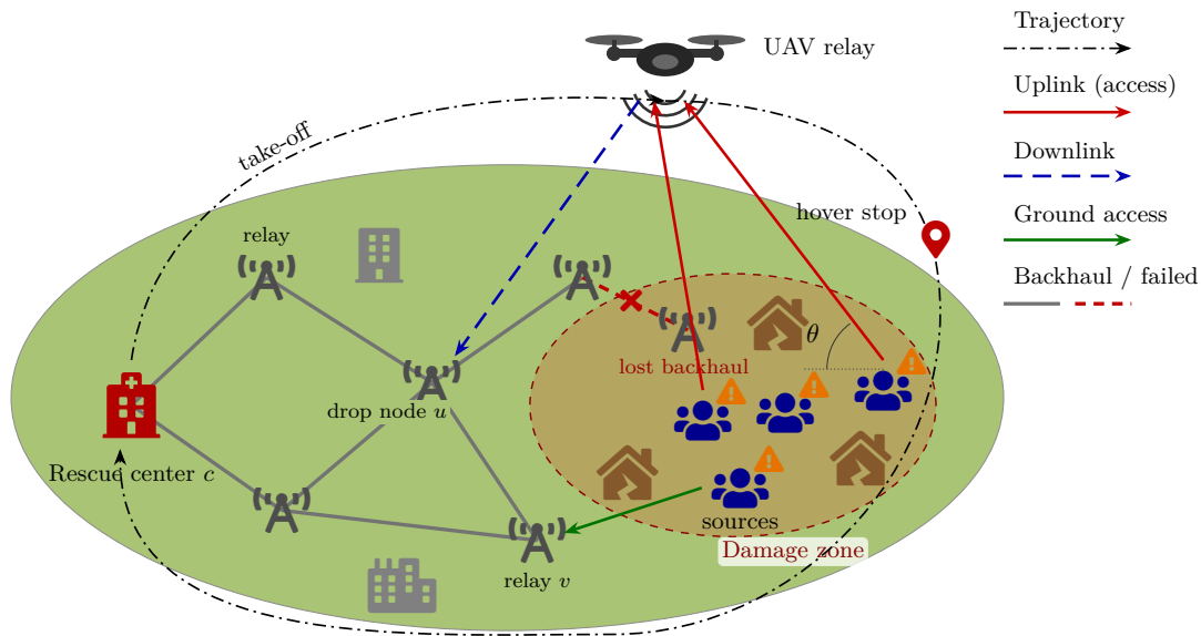
Figure 1. Model of the UAV-assisted alert delivery system.
