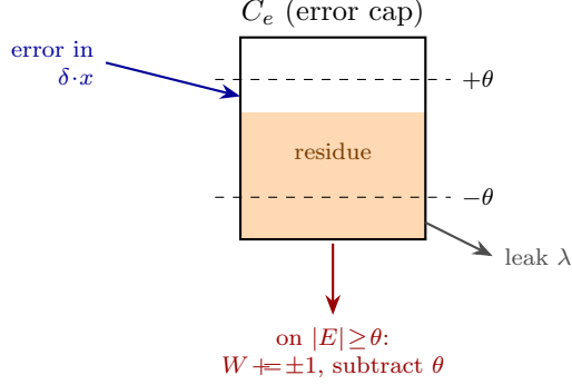
Figure 2: The leaky jug. Error accumulates on the capacitor; it leaks, which supplies momentum; a threshold crossing fires one weight LSB and subtracts \theta , retaining the residue. The retained residue is what makes the mechanism a sigma–delta modulator rather than a lossy quantiser.
