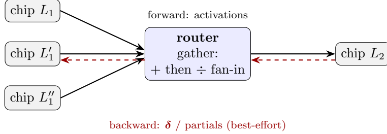
Figure 4: The network. The chips perform all computation; the router only gathers. Forward activations (solid) and error messages (dashed) share the same physical links, so there is no separate backward network. Because the transpose runs on the chips, the router holds no weights: it sums the partials arriving for each destination and divides by the nominal fan-in — an adder tree and a divider. Forward traffic is reliable; error traffic is best-effort.
