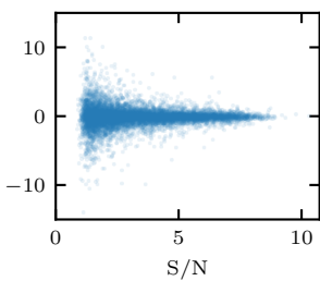
\Delta EW/EW Ca II 8662
