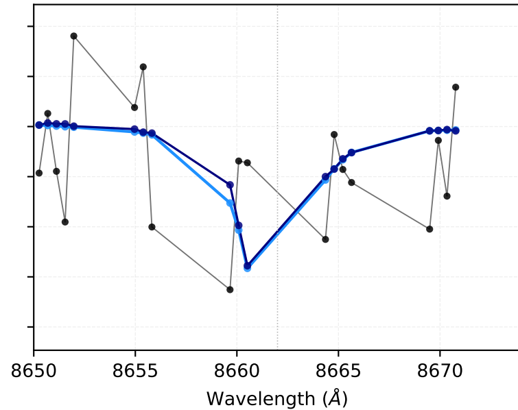
Ca II \lambda 8662
