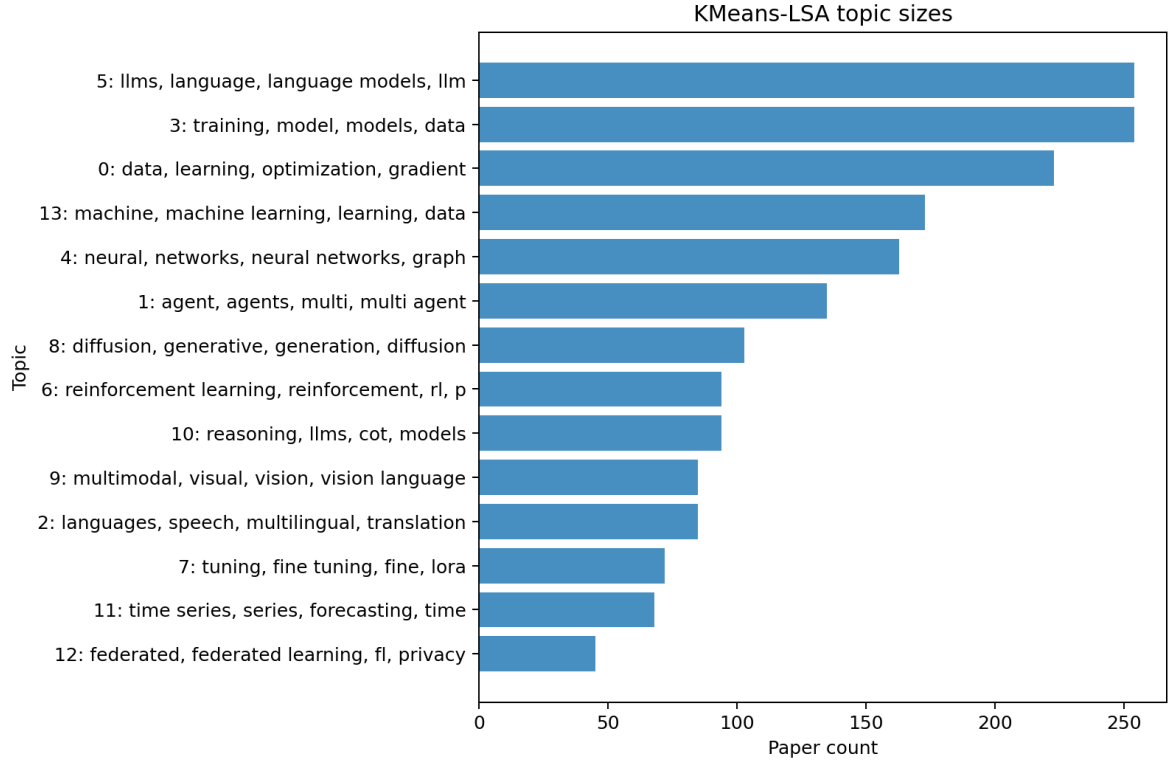
Figure 3: Topic sizes for the selected KMeans-LSA model.
