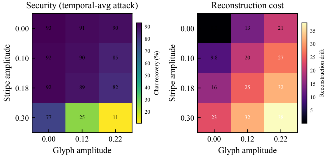
FIGURE 10. Anti-OCR profile stripe \times glyph amplitude grid (temporal-average attack): left panel shows character recovery, right panel shows digital reconstruction drift. High stripe and glyph amplitude regions descriptively reduce character recovery to \sim 11\% across the current 12 parameter grid points (16 samples per point) while increasing reconstruction cost. No significance testing was performed.
