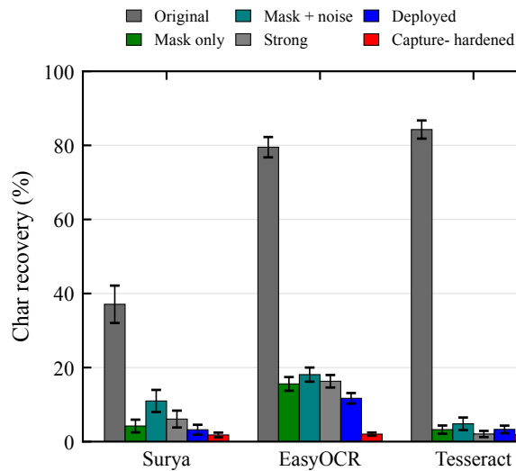
FIGURE 6. Real-capture short-exposure character recovery for three OCR engines across all six profiles in Table 5; error bars are 95% bootstrap intervals resampled by capture. All three engines are suppressed, but with a limited engine family this cannot be claimed as recognizer-agnostic.
