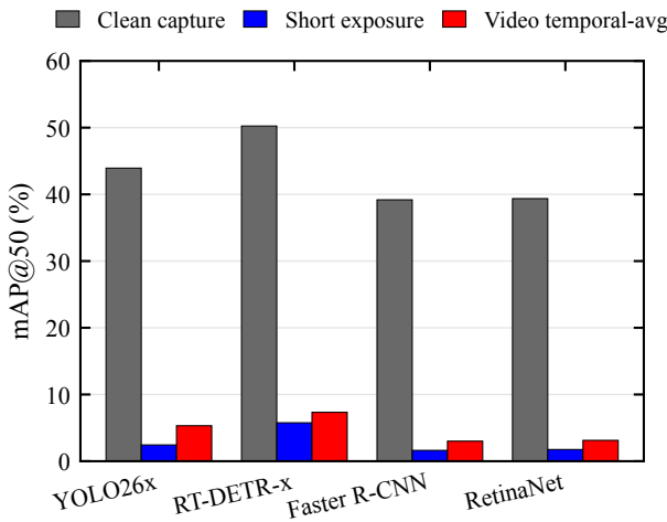
FIGURE 6. Real-capture mAP50 for four detectors across the unprotected capture, short-exposure protected capture, and 150-frame protected mean. Conditions differ in protection, exposure, resolution, and frame reduction.
