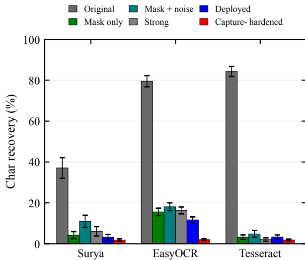
FIGURE 6. Real-capture short-exposure character recovery for three OCR engines across all six profiles in Table 4; error bars are 95% bootstrap intervals resampled by capture. All three engines are suppressed, but with a limited engine family this cannot be claimed as recognizer-agnostic.
