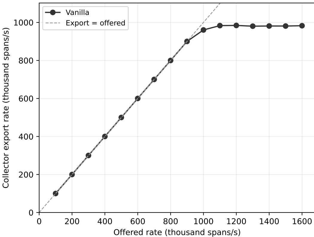
Zero semconv attributes · 1 collector CPU, 4 GiB · PROTO export to /dev/null
