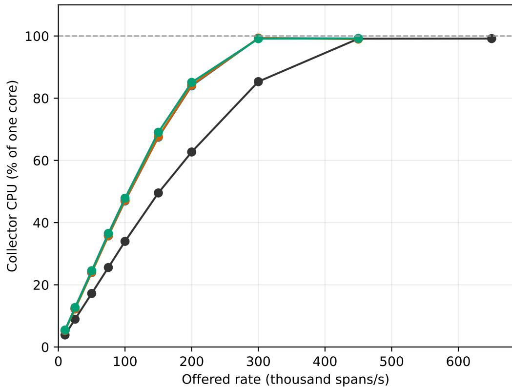
Zero semconv attributes · 1 collector CPU, 4 GiB · JSON export to /dev/null
