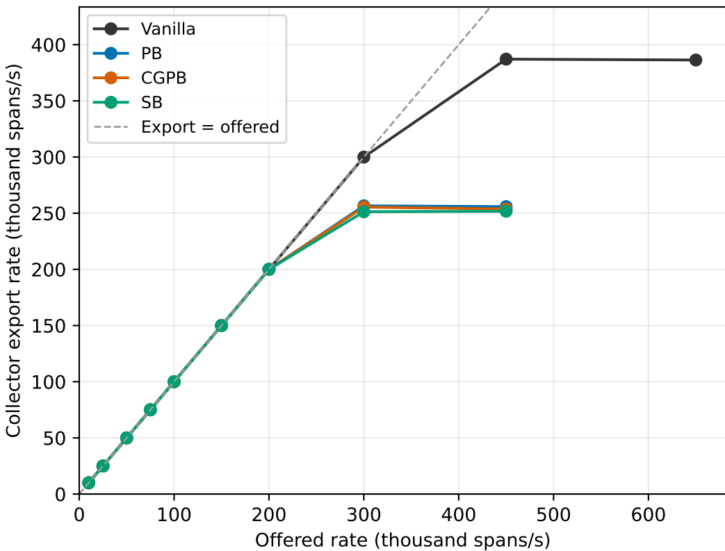
Zero semconv attributes · 1 collector CPU, 4 GiB · JSON export to /dev/null
