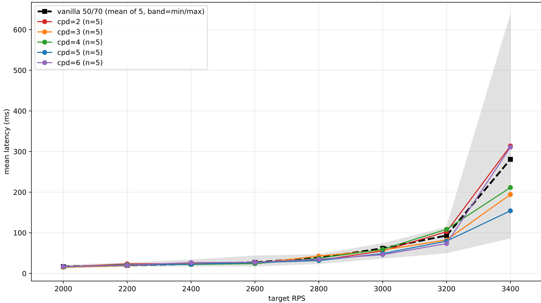
v28: app mean latency vs load (linear, pre-saturation), by cpd
