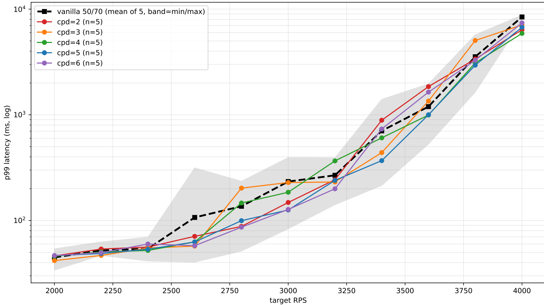
v28: app p99 latency vs load, by cpd (vs vanilla 50/70)
