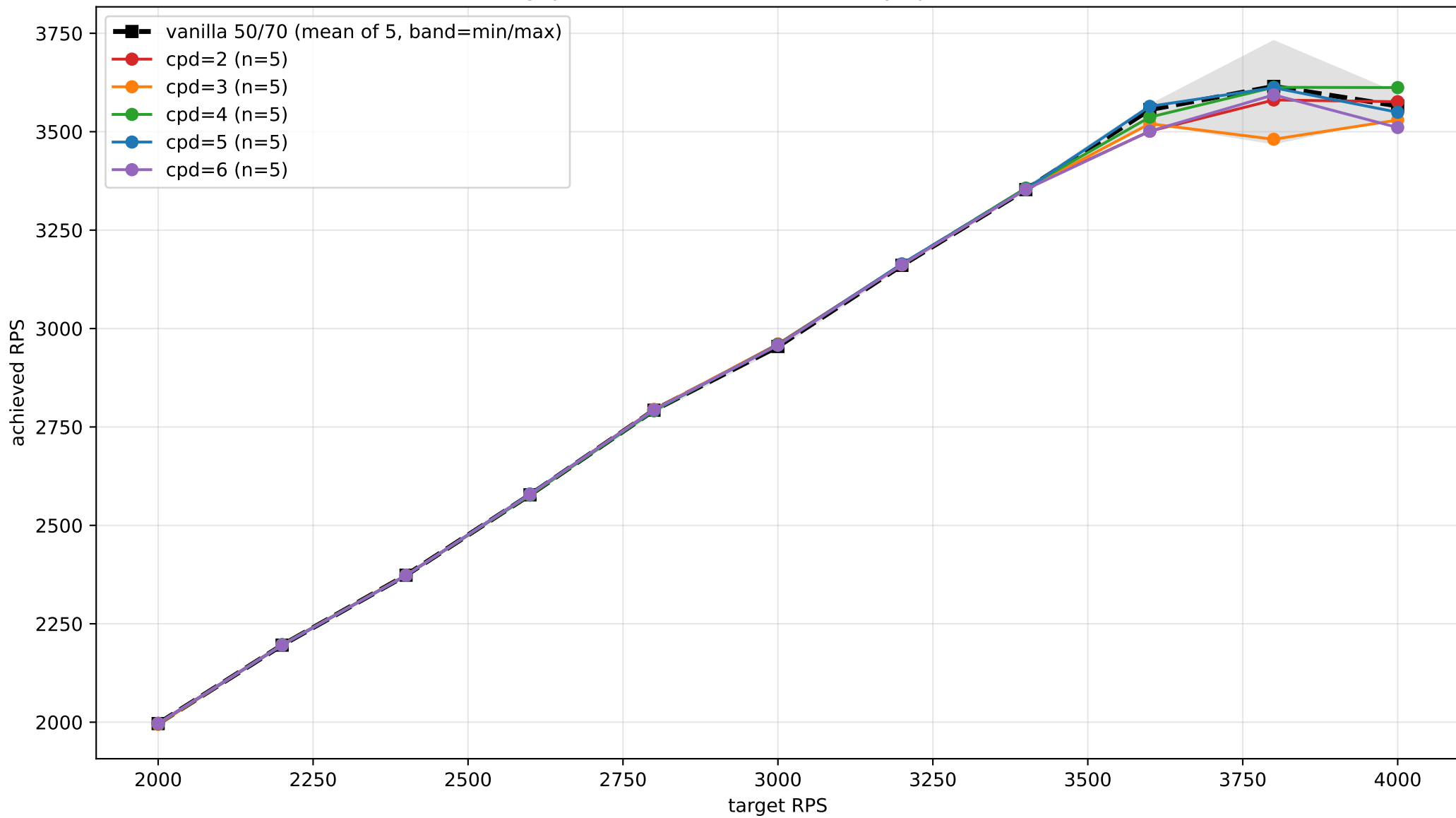
v28: throughput (achieved RPS) vs load, by cpd (vs vanilla 50/70)
