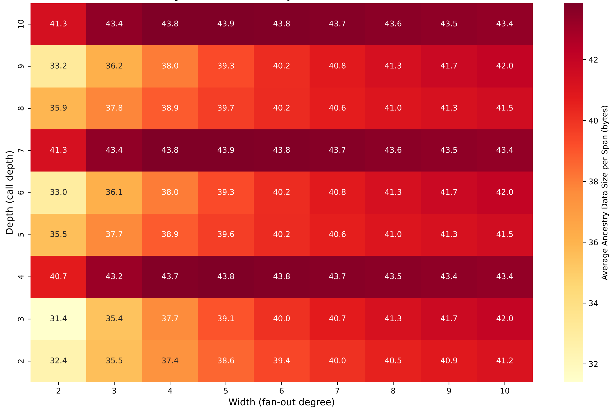
Average Ancestry Data Size per Span (Hybrid mode, checkpoint distance = 3)
