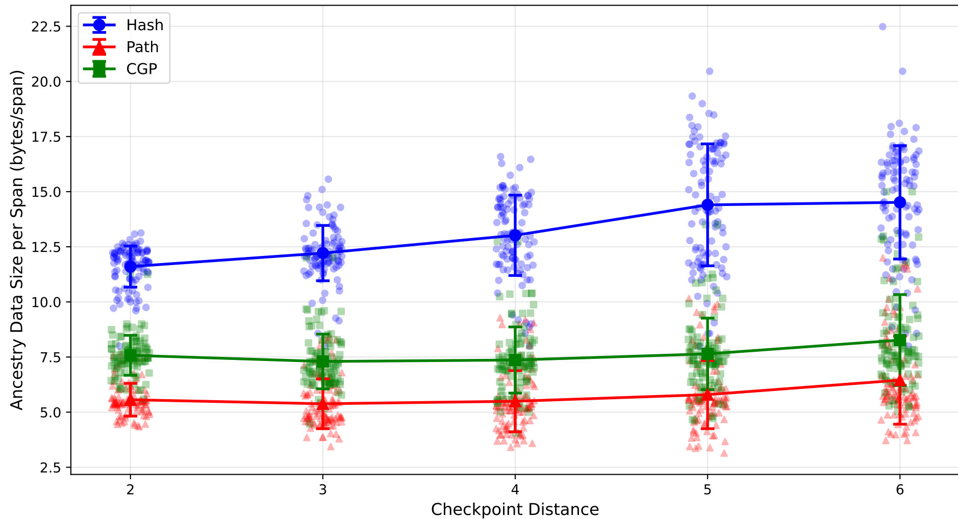
Checkpoint Distance vs Ancestry Data Size per Span (with distribution)
