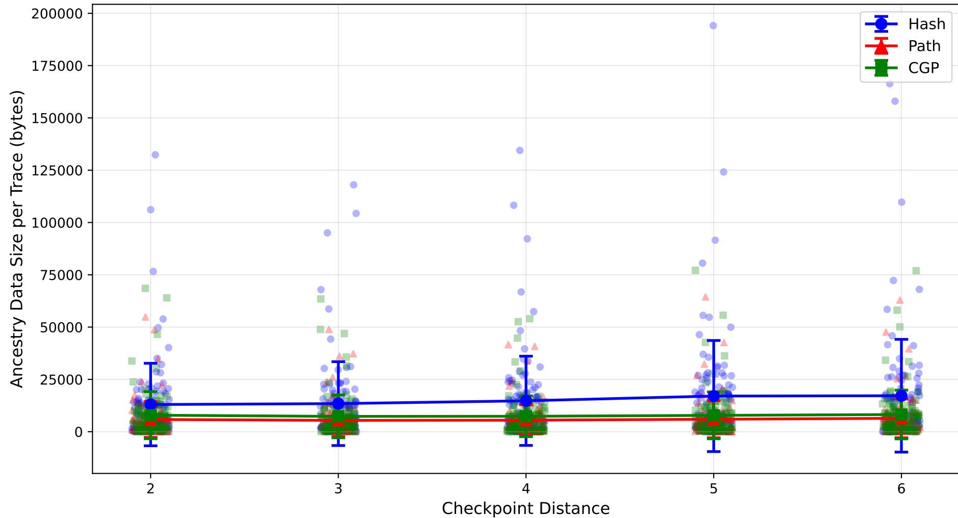
Checkpoint Distance vs Average Ancestry Data Size per Trace (with distribution)
