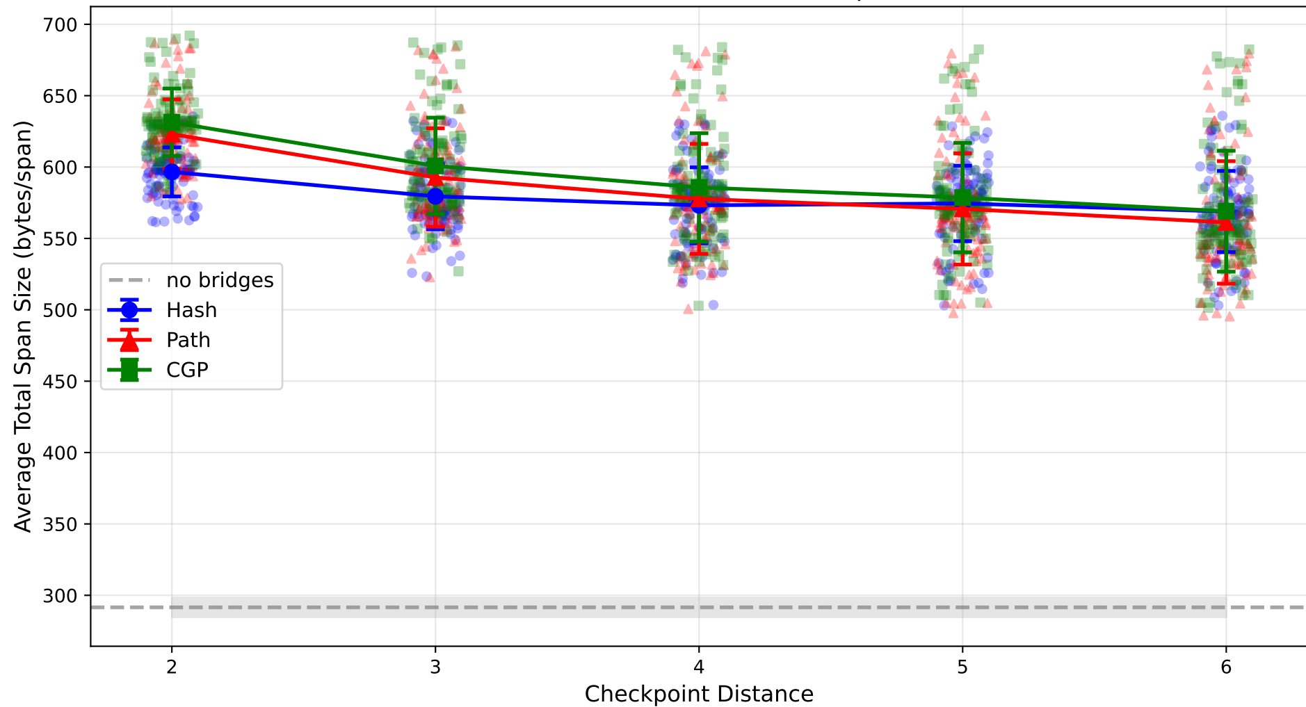
Checkpoint Distance vs Average Total Span Size (total trace size / number of spans)
