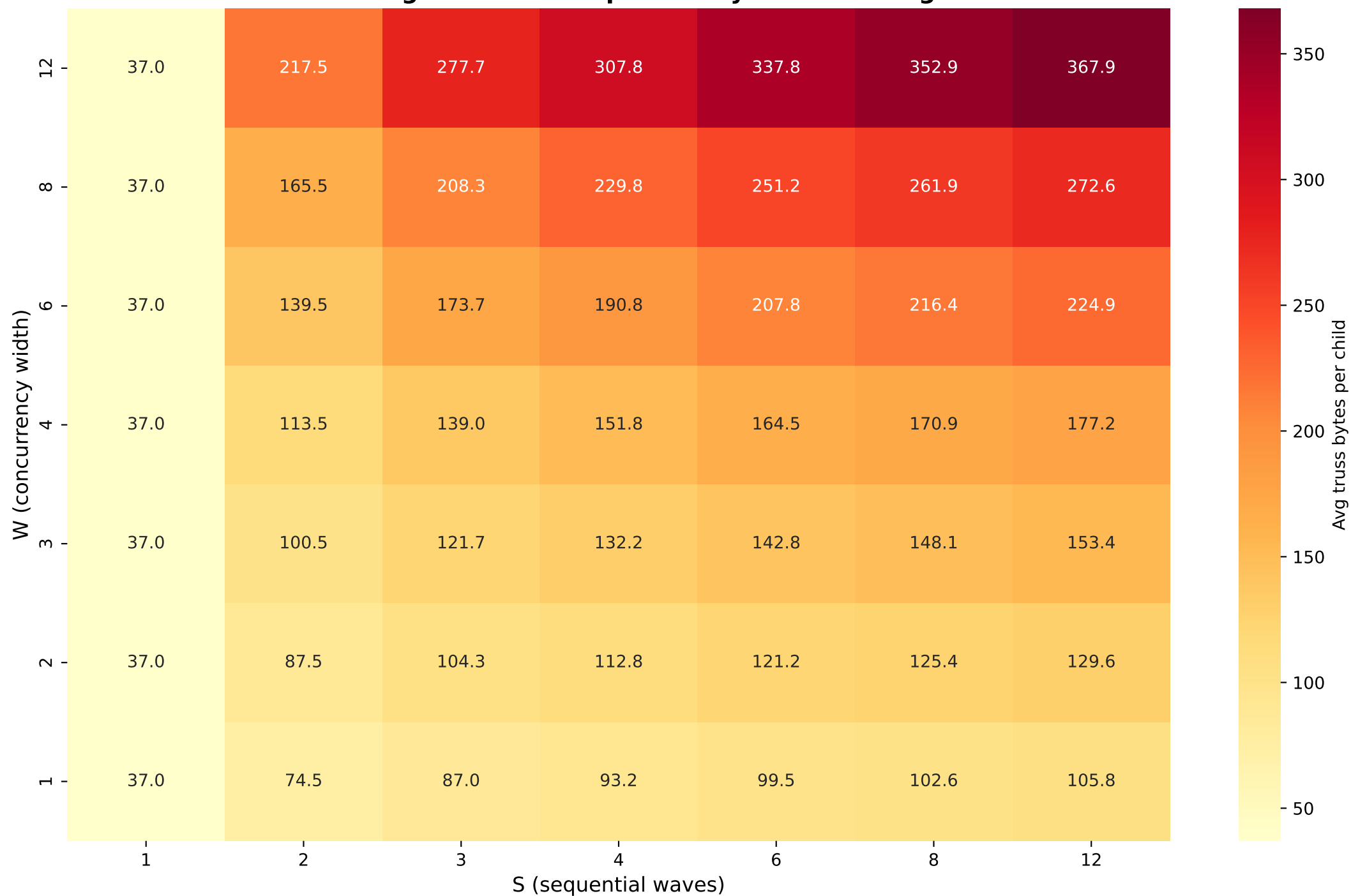
Worst-case avg truss bytes per child Assuming context = all previously ended siblings
