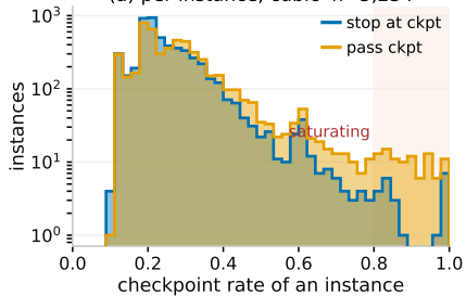
(a) per instance, cubic n=5,234
