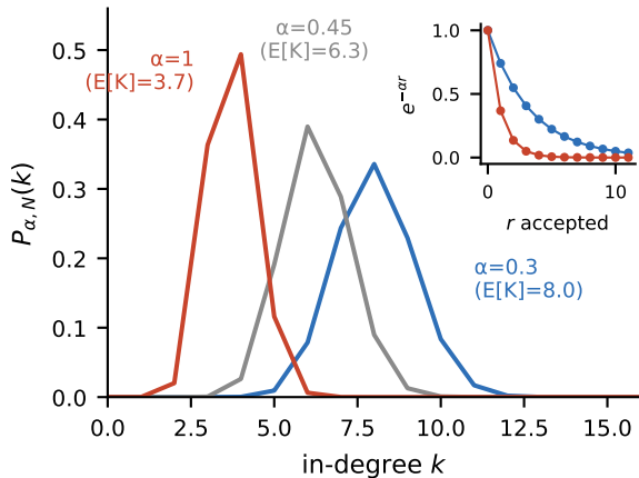
(a) crowding-generated in-degree, N = 32
