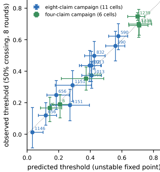
Figure 7: Calibration of threshold predictions (qwen3:8b). Predicted unstable-fixed-point position (per-claim divisive response function) against the observed threshold (50% crossing of the eight-round outcome) for every (claim, \alpha ) cell observed bistable: circles, the eight-claim campaign (11 cells); squares, the four-claim campaign (6 cells). Vertical bars are episode-bootstrap 95% intervals of the observed threshold, horizontal bars are single-agent-bootstrap 95% intervals of the prediction, and the dotted line is identity. Cells predicted and observed monostable (4 of 16 and 6 of 12) and the one class mismatch (claim 1146 at \alpha = 0.30 ) are listed in the SI.
