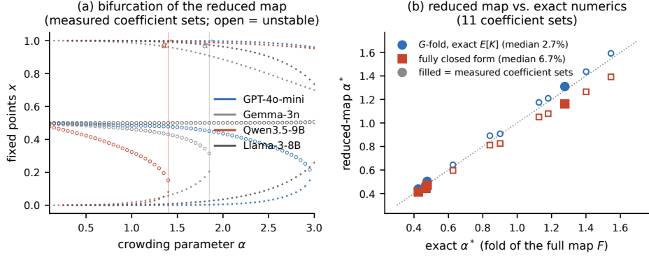
Figure 2: Critical crowding level from the reduced map. (a) Fixed points of the reduced map G as functions of \alpha for the four measured coefficient sets of El et al. (2026a); the interior unstable branch (open symbols) vanishes at \alpha^* . (b) Validation of the two closure levels against the fold of the full map F over 11 coefficient sets (filled symbols: coefficient sets measured in this study).
