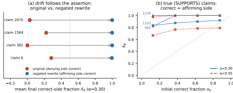
Figure 5: Final correct-side fractions for original, negated, and true claims. (a) Mean final correct-side fraction for the four original claims (denying side correct) and their minimally negated rewrites (affirming side correct) under identical conditions: the content-referenced outcome reverses with the wording. (b) True (SUPPORTS) claims converge on the correct = affirming side from all initial fractions.
