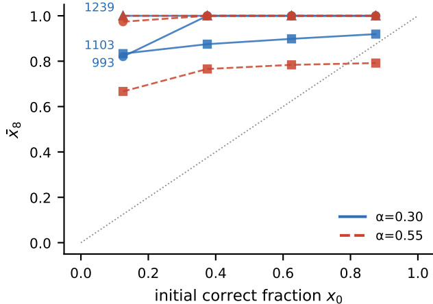
(b) true (SUPPORTS) claims: correct = affirming side
