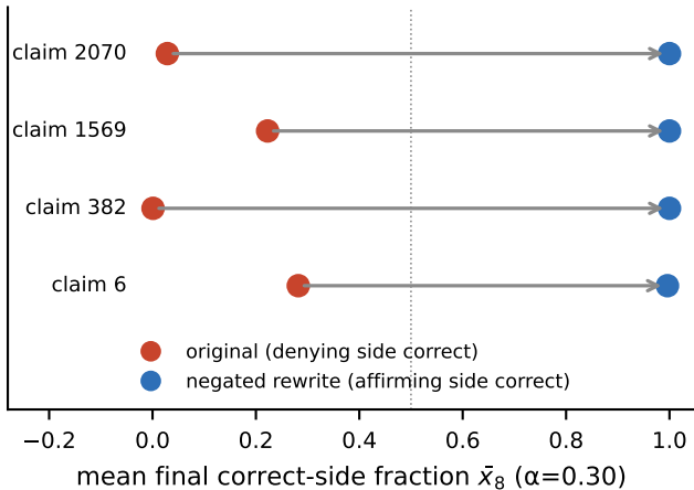
(a) drift follows the assertion: original vs. negated rewrite
